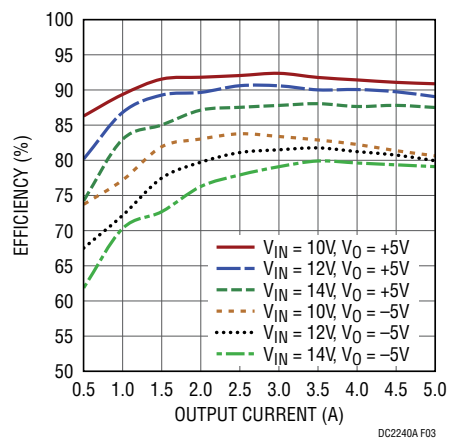
Figure 3. Typical Efficiency Curve
