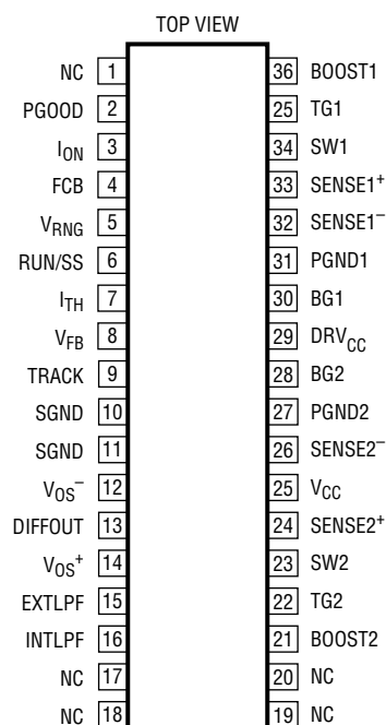
G PACKAGE 36-LEAD PLASTIC SSOP T_{JMAX} = 125^{\circ}\text{C} , \theta_{JA} = 95^{\circ}\text{C/W}
