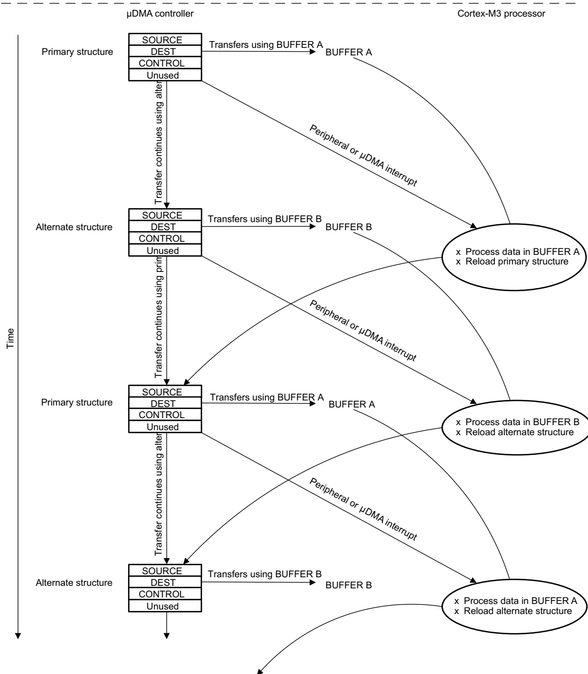
Figure 12-2. Example of Ping-Pong \mu DMA Transaction
