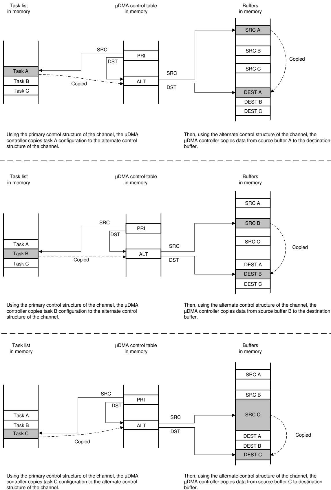
Figure 12-4. Memory Scatter-Gather, \mu DMA Copy Sequence
