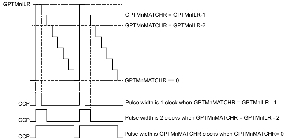
Figure 13-7. CCP Output, GPT:TnILR > GPT:TnMATCHR
