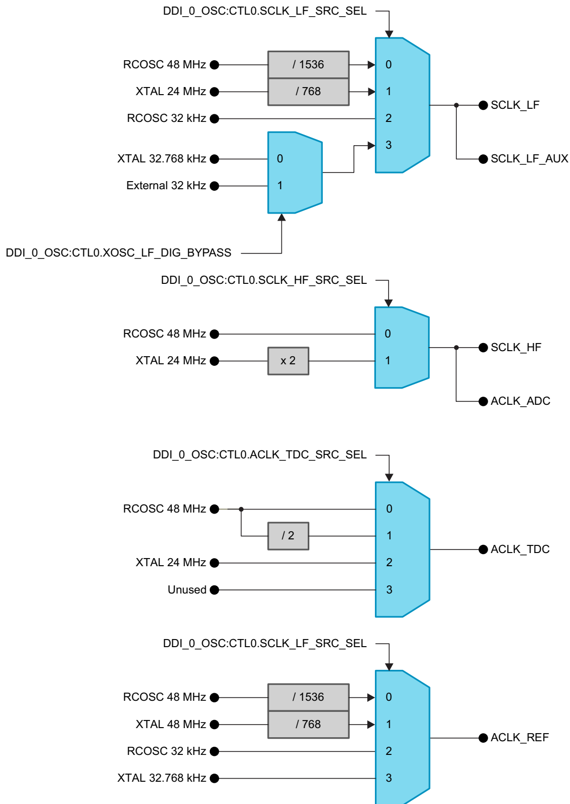
Figure 6-5. System Clock Muxing
