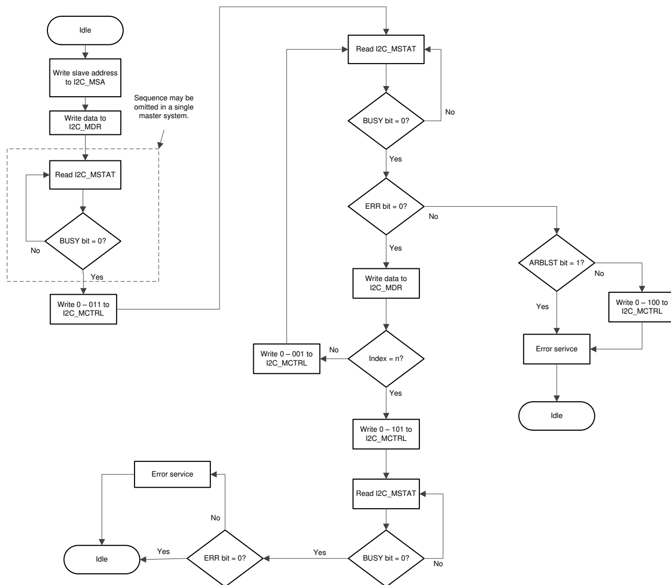
Figure 21-9. Master TRANSMIT With Repeated Start Condition
