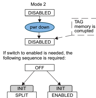
Figure 7-7. GPRAM Retention
