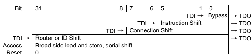
Figure 5-4. Data Shift Register
