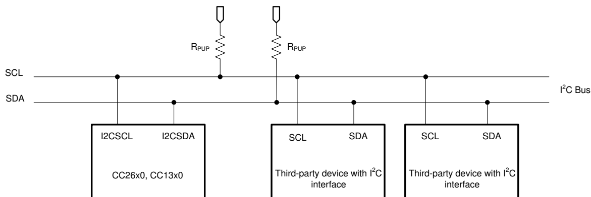
Figure 21-2. I 2 C Bus Configuration
