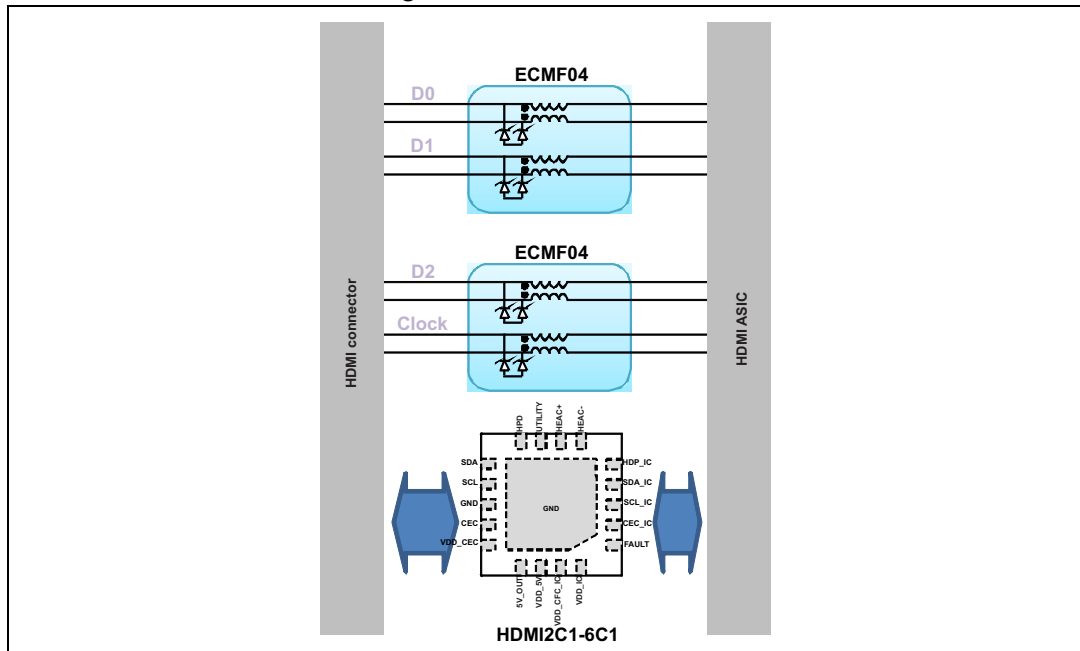
Figure 15. HDMI schematic
