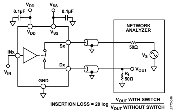
Figure 39. Bandwidth
