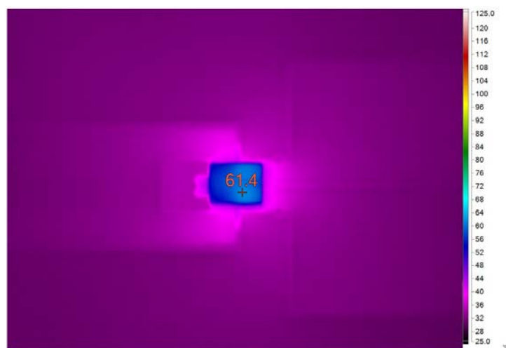
Figure 9. Thermal performance at V_{IN} = 3.3V , V_{OUT1} = 1.2V , V_{OUT2} = 1.8V , I_{OUT1} = 2A , I_{OUT2} = 2A T_A = 23^\circ C , No Forced Airflow
