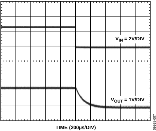
Figure 7. Turn-Off Time with a 1 \mu F Input Capacitor
