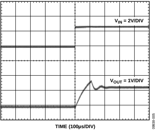
Figure 5. Turn-On Time with a 1 \mu F Input Capacitor
