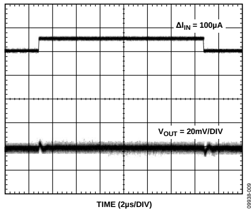
Figure 9. Output Response to a 100 \mu\text{A} Input Current Change with a 1 \mu\text{F} Capacitor
