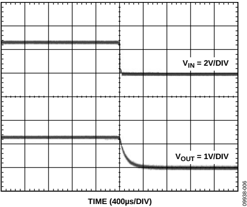
Figure 6. Turn-Off Time
