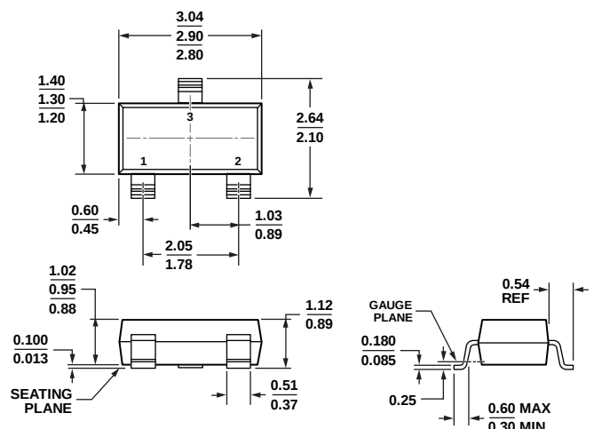
Figure 15. 3-Lead Small Outline Transistor Package [SOT-23-3] (RT-3)
