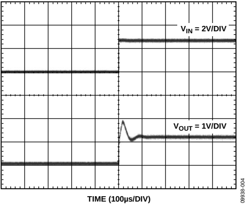
Figure 4. Turn-On Time
