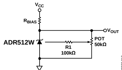
Figure 12. Output Voltage Trim
