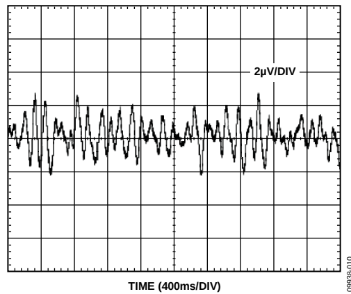
Figure 10. 0.1 Hz to 10 Hz Noise
