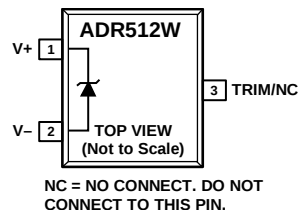
Figure 1. 3-Lead SOT-23
