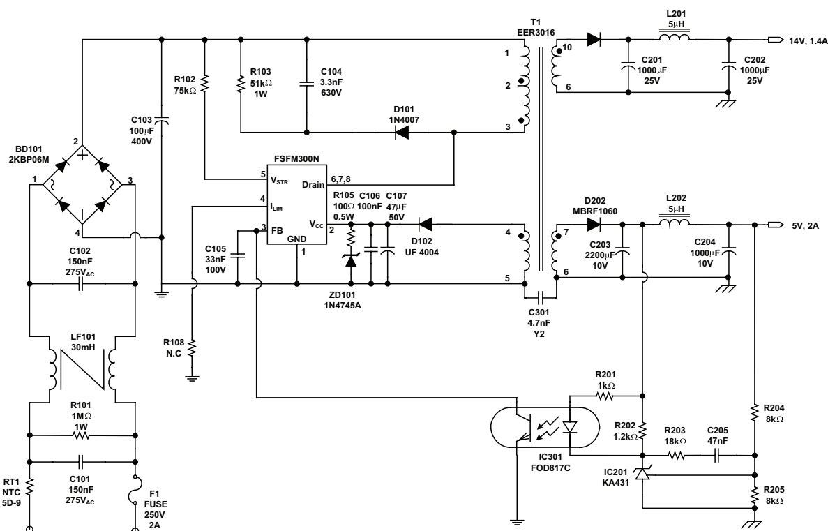
Figure 24. Demonstration Circuit of FSFM300N
