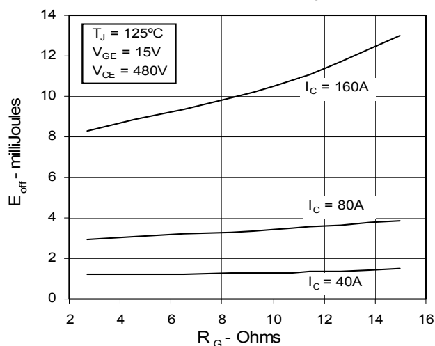
Fig. 8. Dependence of Turn-off Energy Loss on R_G
