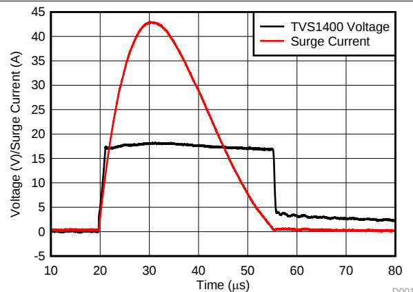
Figure 11. TVS1400 Clamping Response at 43 A
