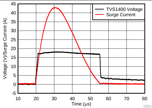
Figure 1. Surge Response at 43 A
