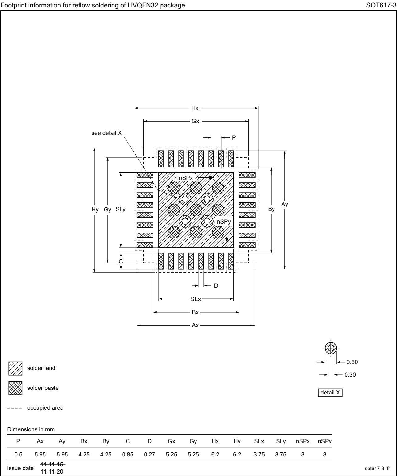
Fig 9. PCB footprint for SOT617-3 (HVQFN32); reflow soldering
