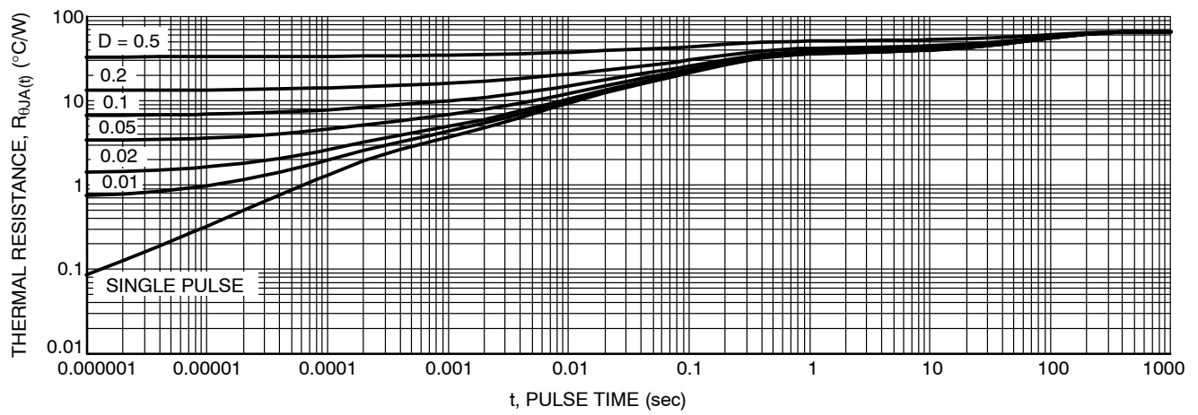
Figure 26. Thermal Response
