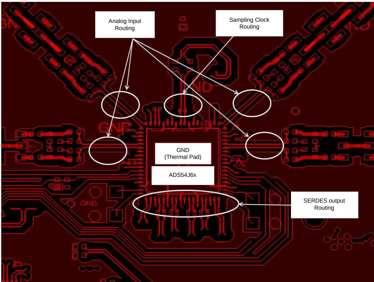
Figure 136. ADS54J64EVM Layout
