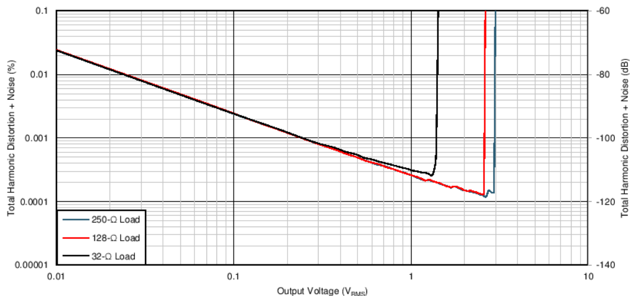
Figure 4. THD+N vs. Amplitude for a 32-, 128-, and 250- \Omega Load
