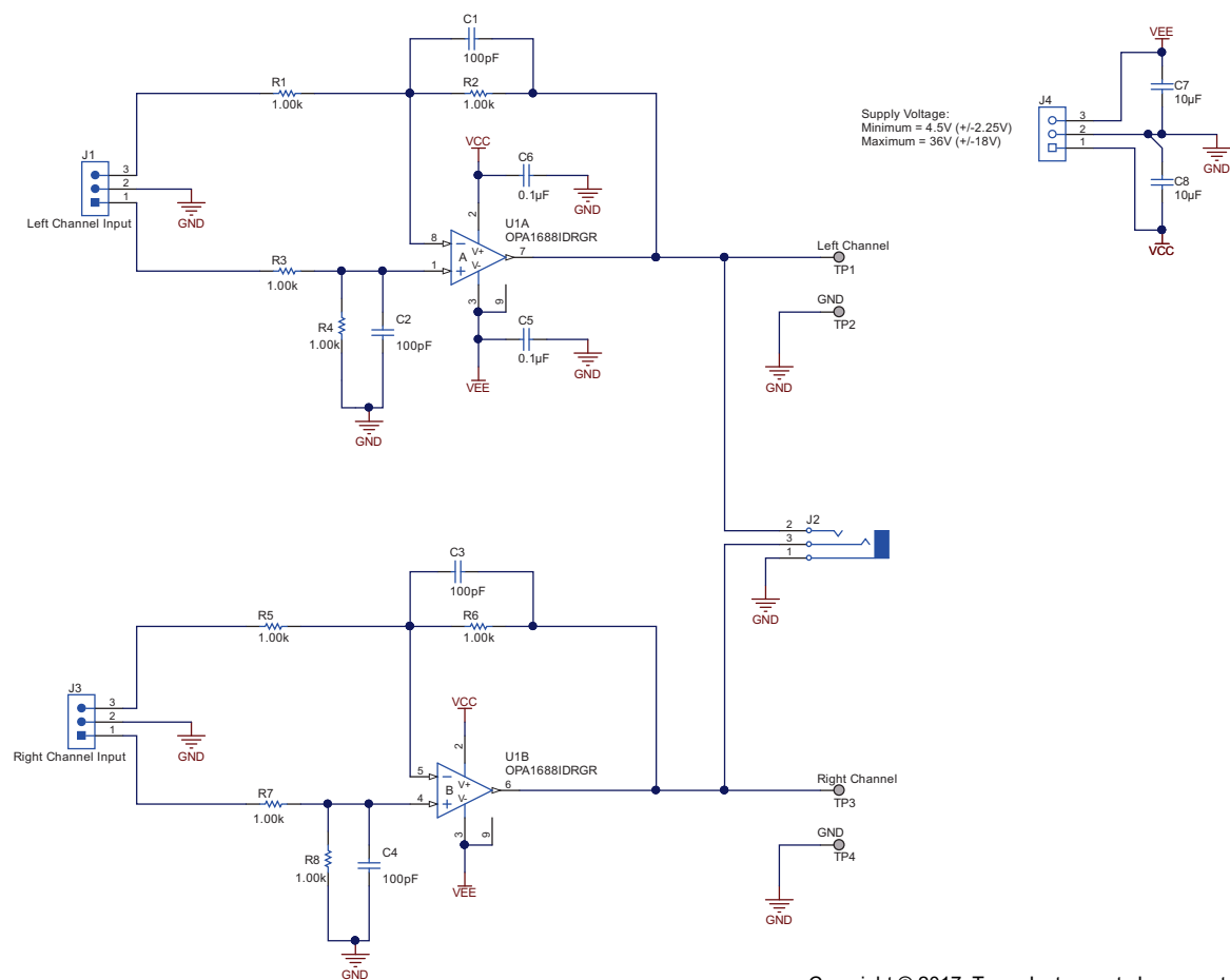
Figure 10. OPA1688EVM Schematic
