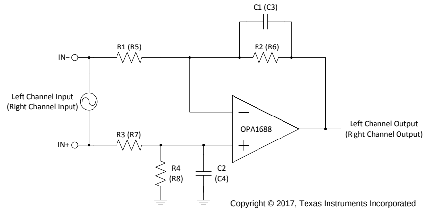
Figure 1. OPA1688EVM Schematic
