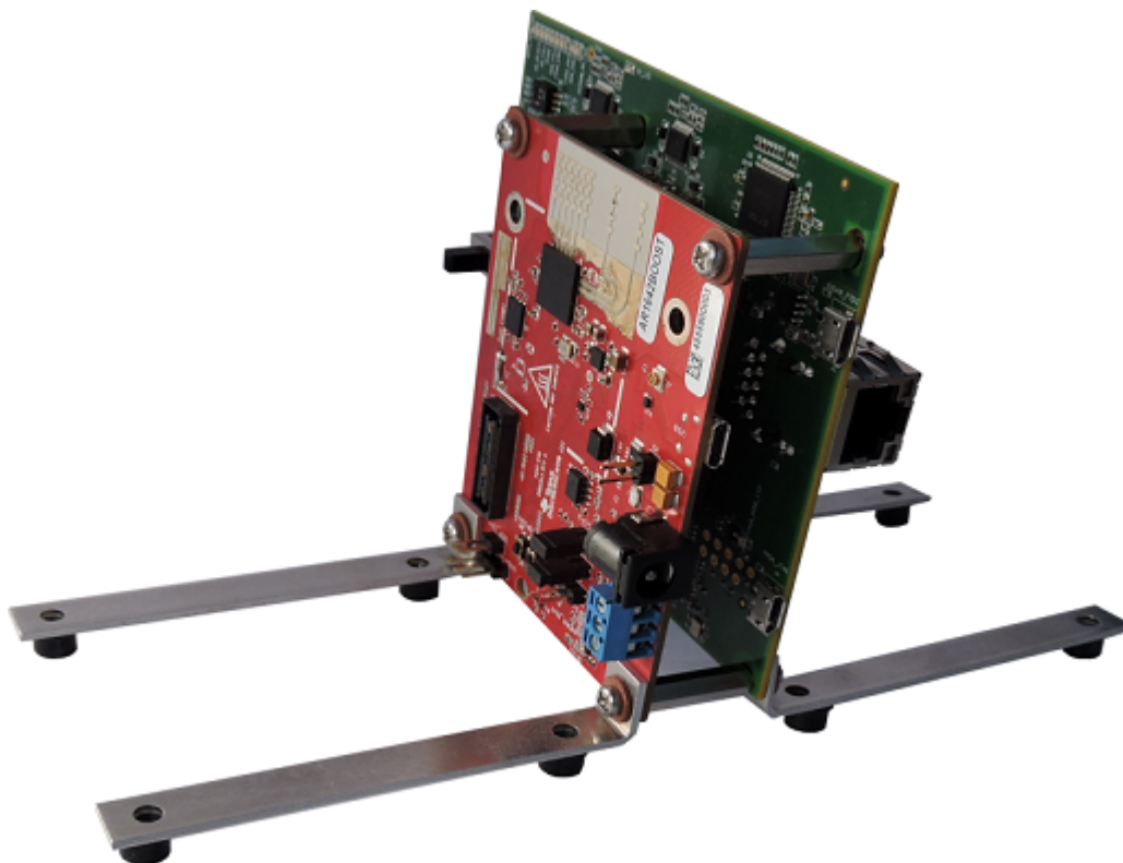
Figure 6. Connect Boards
