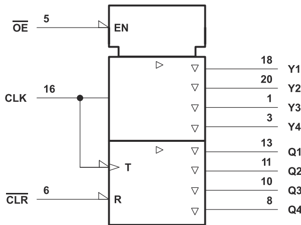
Logic Symbol
