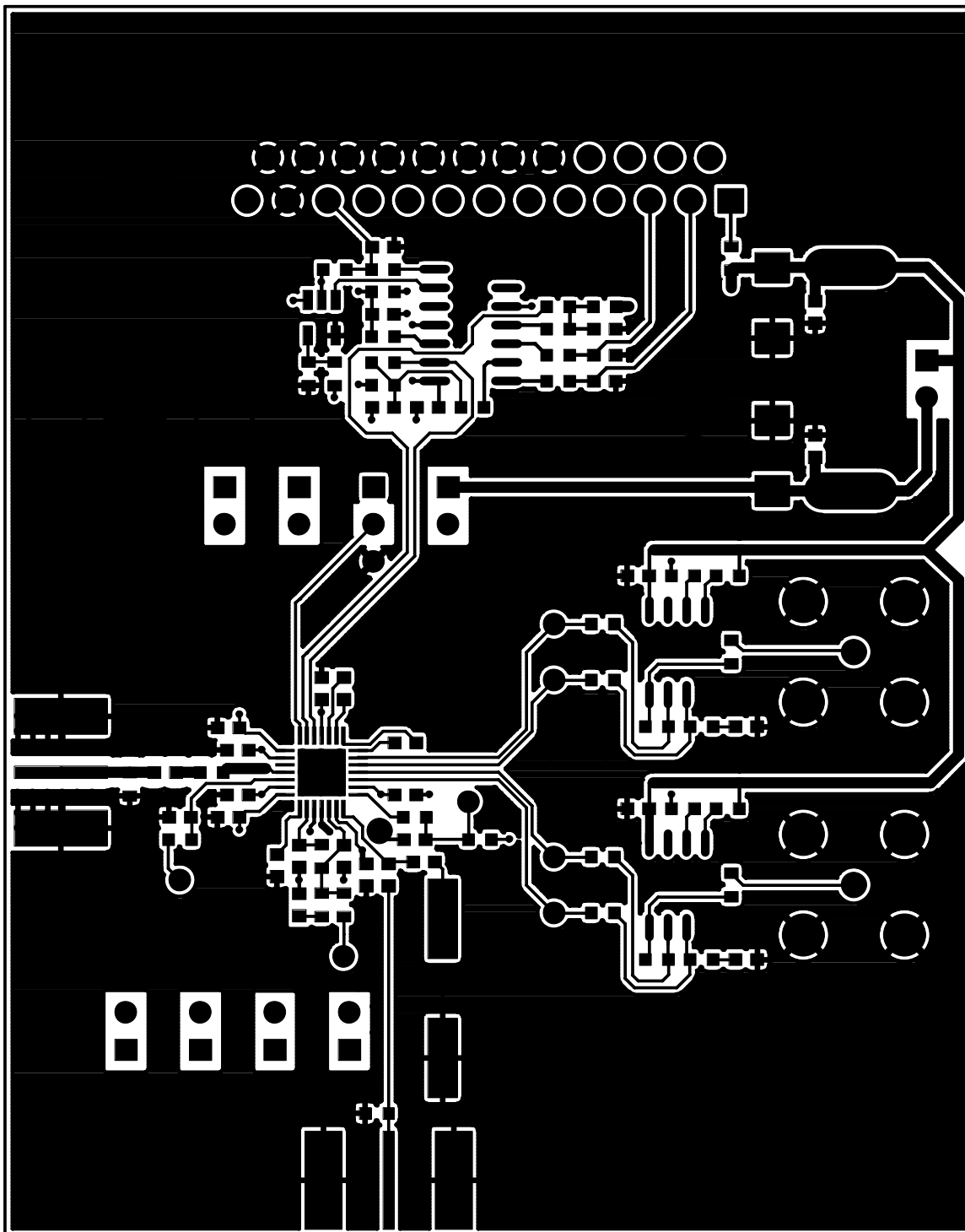
Figure 3. MAX2117 EV Kit PCB Layout—Top
