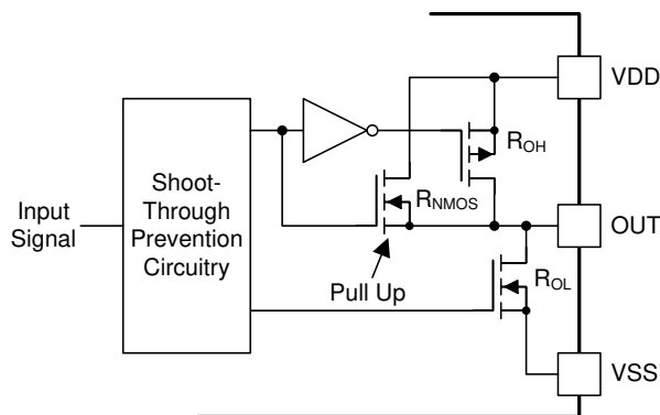
Figure 35. Output Stage
