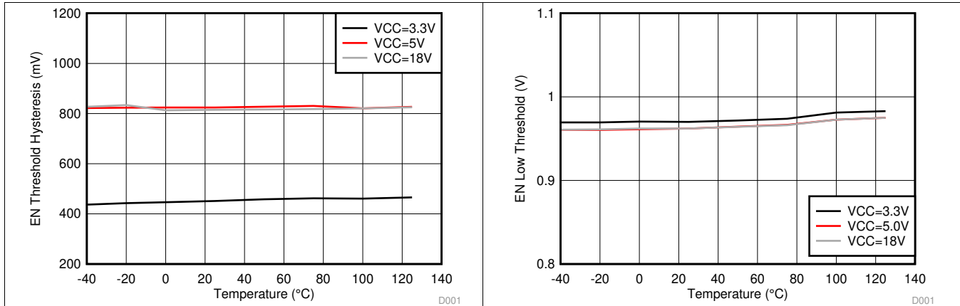
Figure 22. EN Threshold Hysteresis vs. Temperature
