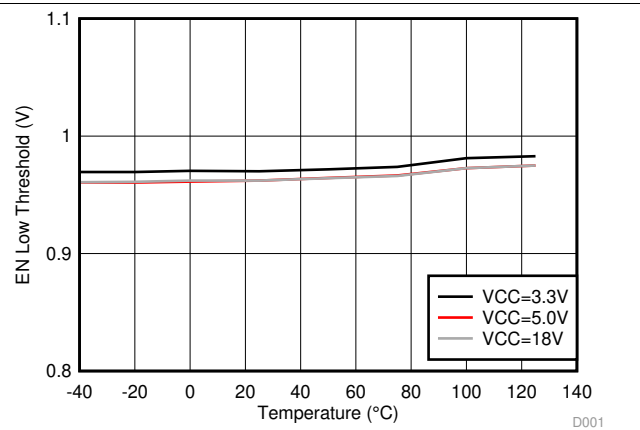
Figure 23. EN Low Threshold
