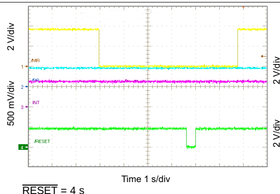
Figure 101. \overline{\text{RESET}} Timing
