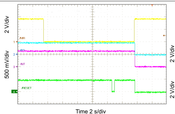
Figure 102. \overline{\text{RESET}} Timing
