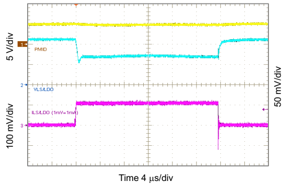
Figure 89. 1.2 V_{SLSDO} Load Transient, 0 to 100 mA
