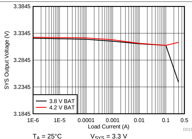
Figure 55. 3.3 V_{SYS} Load Regulation
