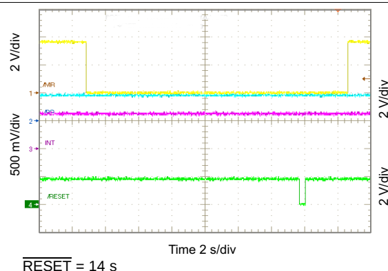
Figure 103. \overline{\text{RESET}} Timing
