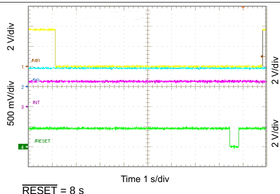
Figure 102. \overline{\text{RESET}} Timing
