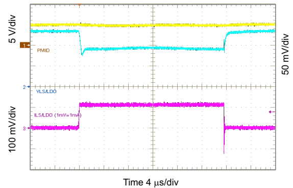
Figure 92. 3.3 V_{SLSDO} Load Transient, 0 to 100 mA
