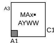
9-Pin Flip-Chip CSP FC SUFFIX CASE 499E
