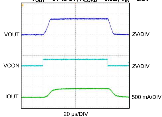
VCON Transient (3G/4G) V_{OUT} = 0V to 3V , R_{LOAD} = 6.8\Omega , V_{IN} = 3.8V
