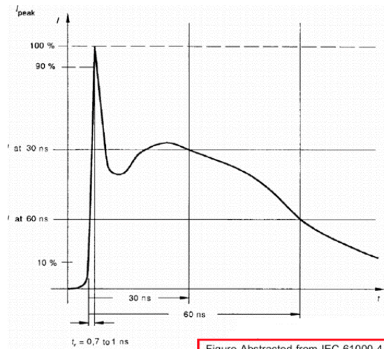
Figure Abstracted from IEC 61000-4-2 © IEC 1995, 1998, 2000
