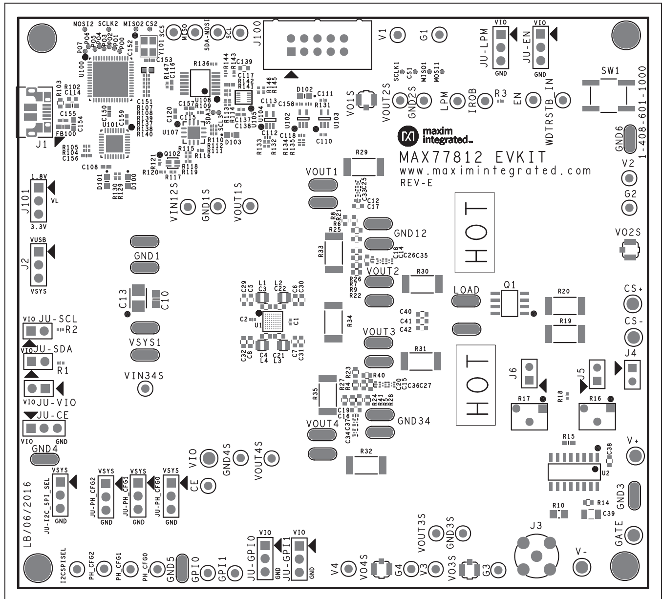
MAX77812 EV Kit Component Placement Guide—Top Silkscreen
