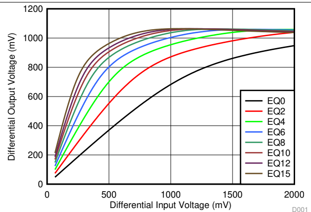
Figure 4. DisplayPort Linearity Curves at 4.05 GHz
