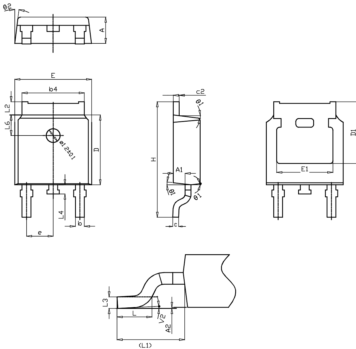
Figure 20. DPAK (TO-252) type C package outline
