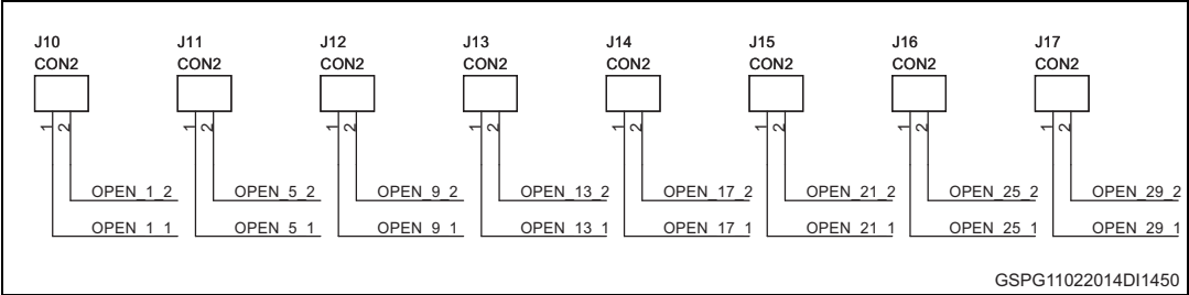
Figure 3. Jumpers to simulate open circuit
