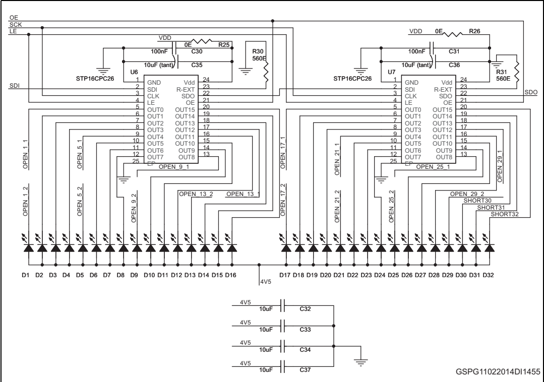
Figure 4. LED driver
