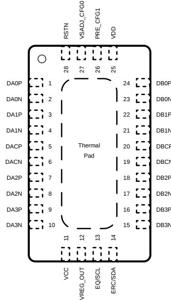
Pin Functions
