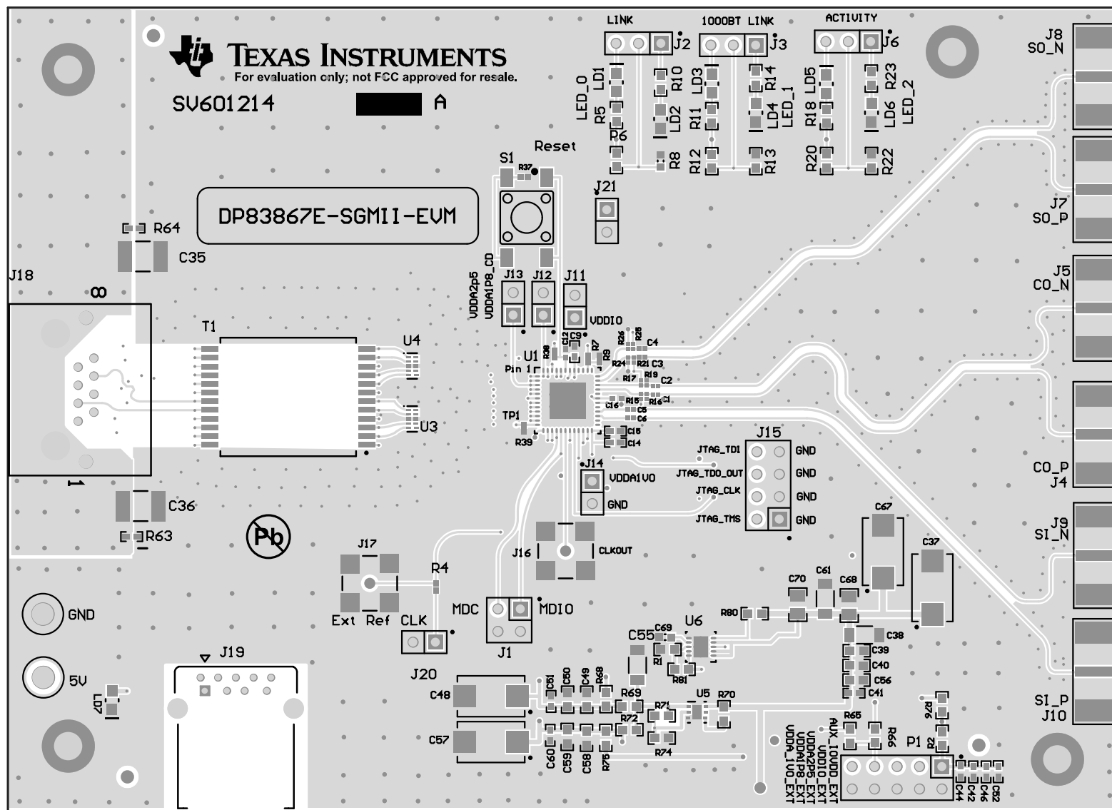
Figure 18. Top Overlay
