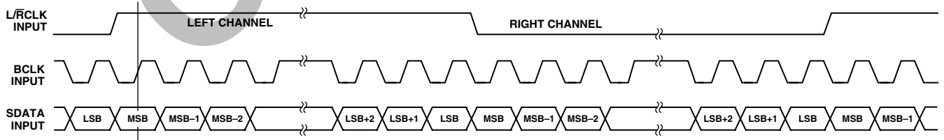
Figure 5. 32 x F s Packed Mode
