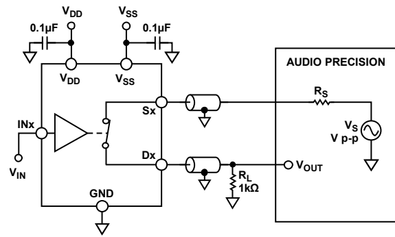
Figure 28. THD + Noise
