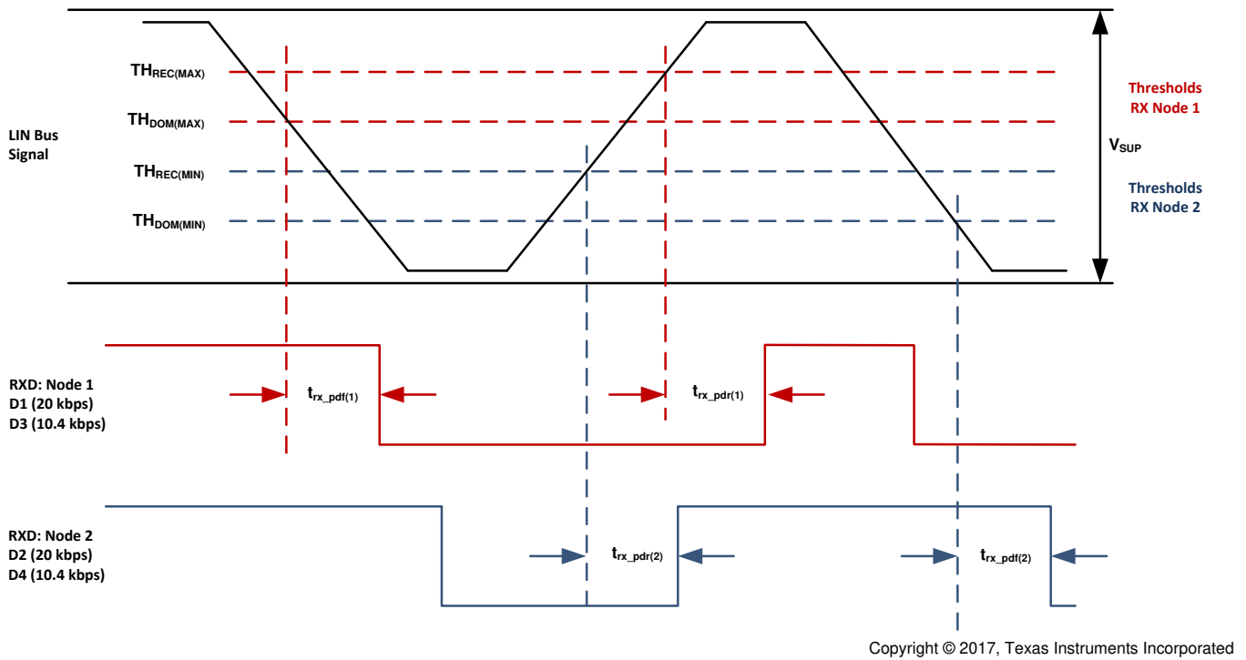
Figure 20. Propagation Delay
