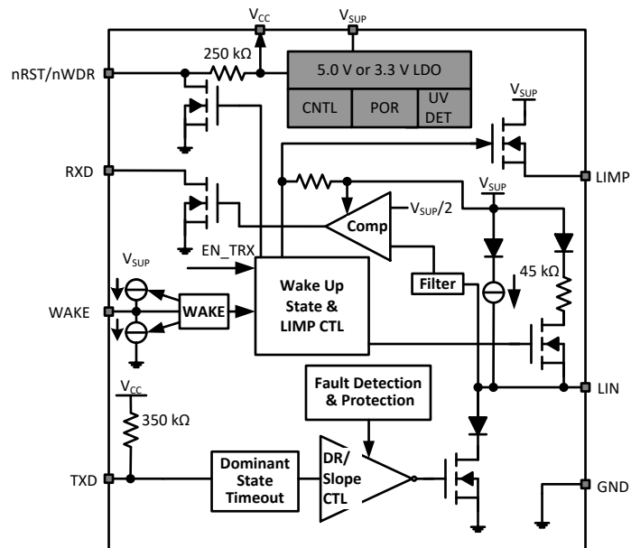
Figure 26. Transceiver plus VREG Functional Block Diagram
