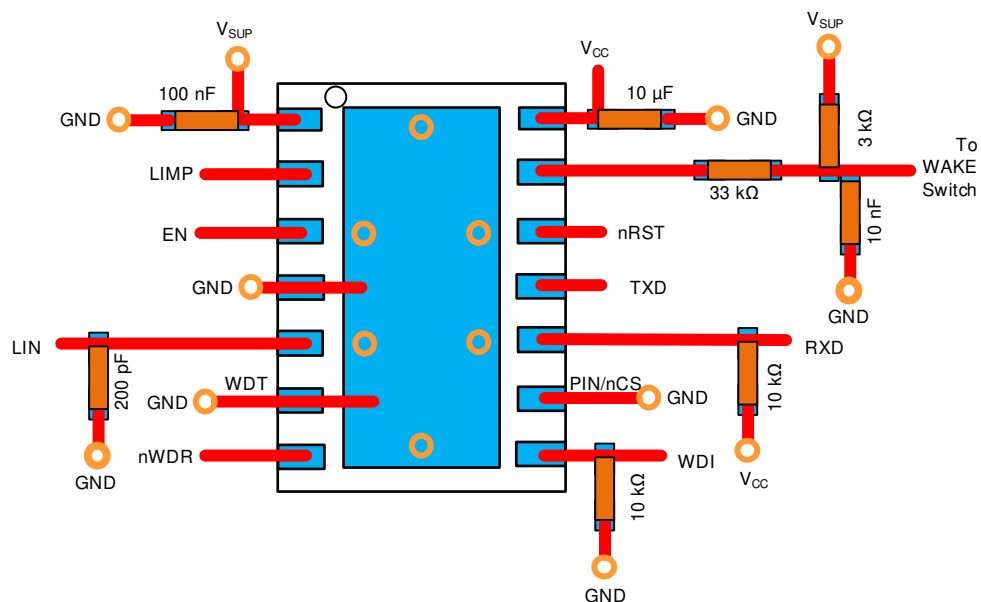
Figure 51. Layout Example
