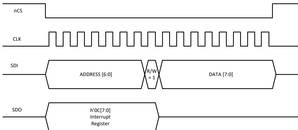
Figure 36. SPI Write
