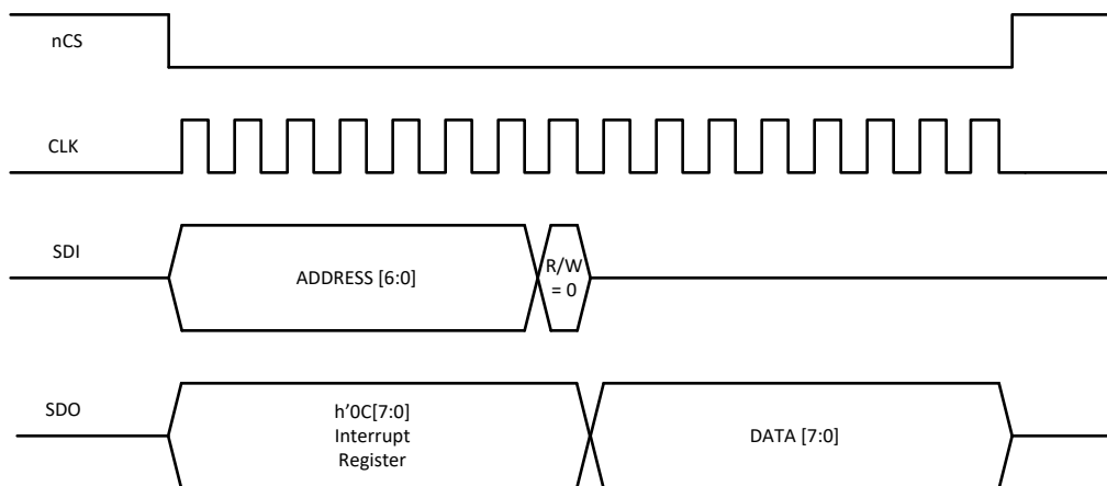
Figure 37. SPI Read
