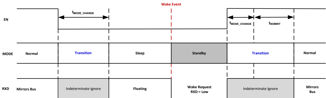
Figure 21. Mode Transitions
