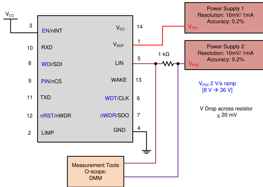
Figure 14. Test Circuit for I_{BUS\_PAS\_rec}
