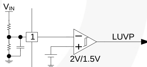
Figure 25. Line UVP Circuit
