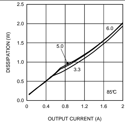
Figure 22. Dissipation 42-V Input, T_A = 85^\circ\text{C}
