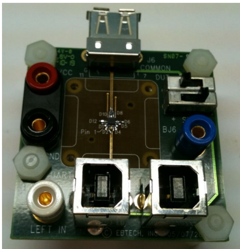
Figure 1. Board Picture
