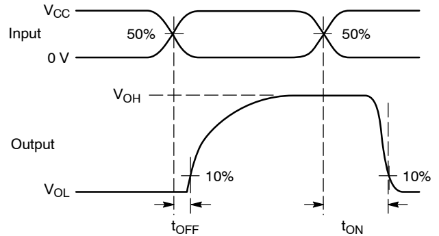
Figure 6. t_{\text{ON}}/t_{\text{OFF}}
