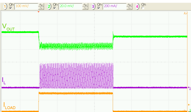
Figure 27. Load Transient 0 to 150 mA, 3.6 V_{IN}
