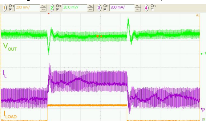
Figure 29. Load Transient 150 to 400 mA, 3.6 V_{IN}
