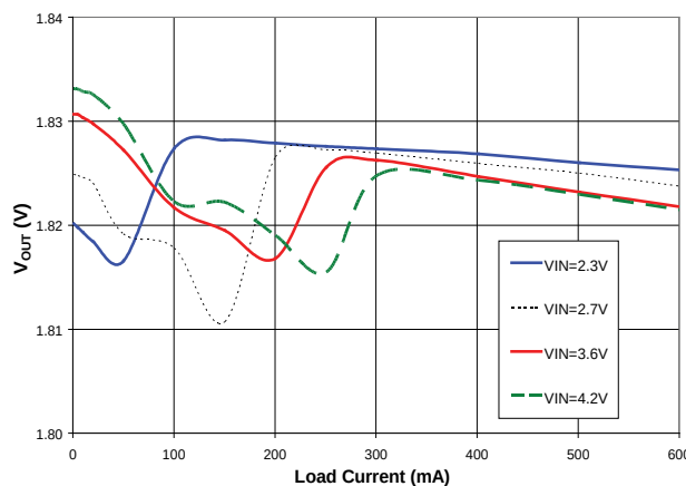
Figure 9. Load Regulation
