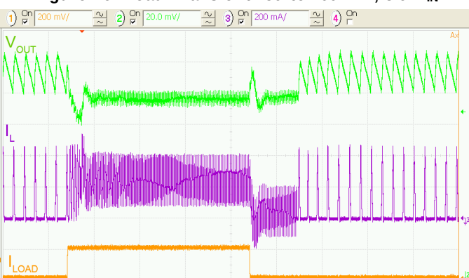
Figure 31. Load Transient 50 to 250 mA, 4.5 V_{IN}
