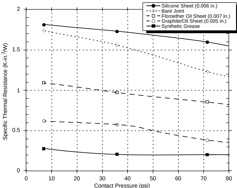
Figure 29. Thermal Performance of Select Thermal Interface Material
