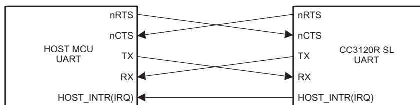
Figure 4-17. Typical 5-Wire UART Topology
