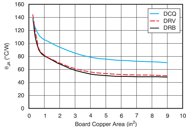
Figure 36. \theta_{JA} vs Board Size
