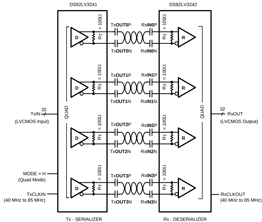
Figure 2. Quad Mode
