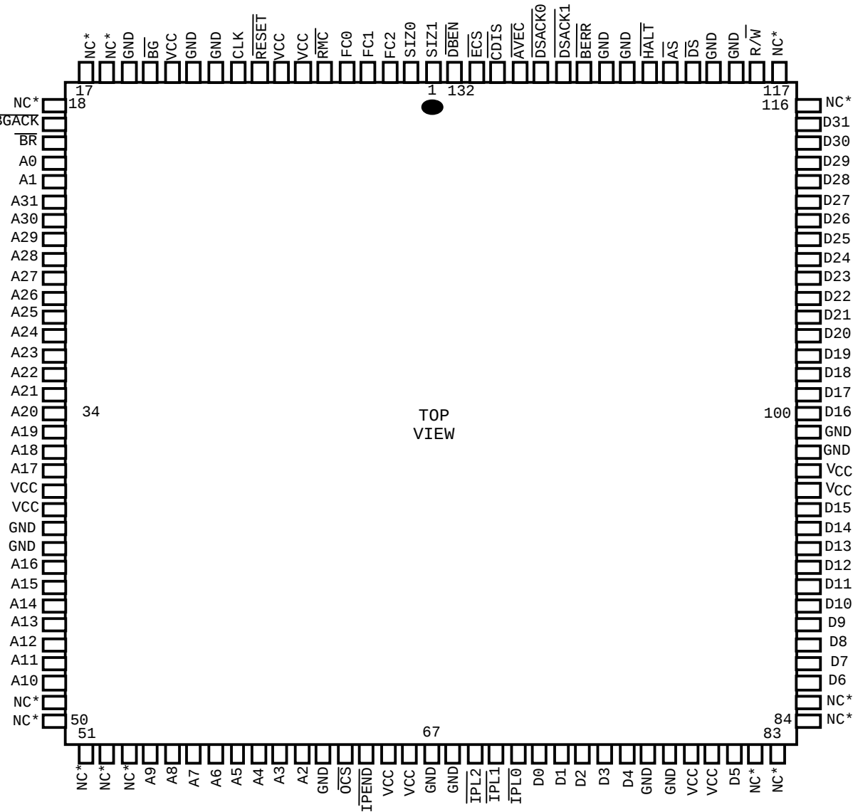
Figure 1. FC and FE Suffix Pin Assignment
