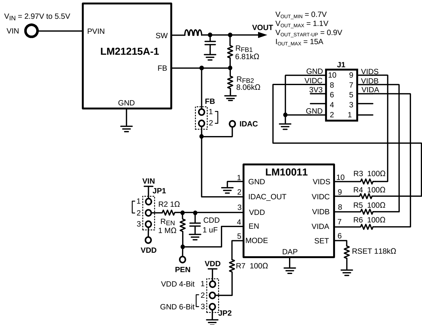
Figure 1. Simplified Schematic
