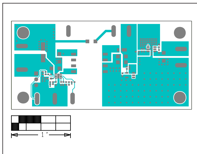
MAX17681A EV Kit—Top
