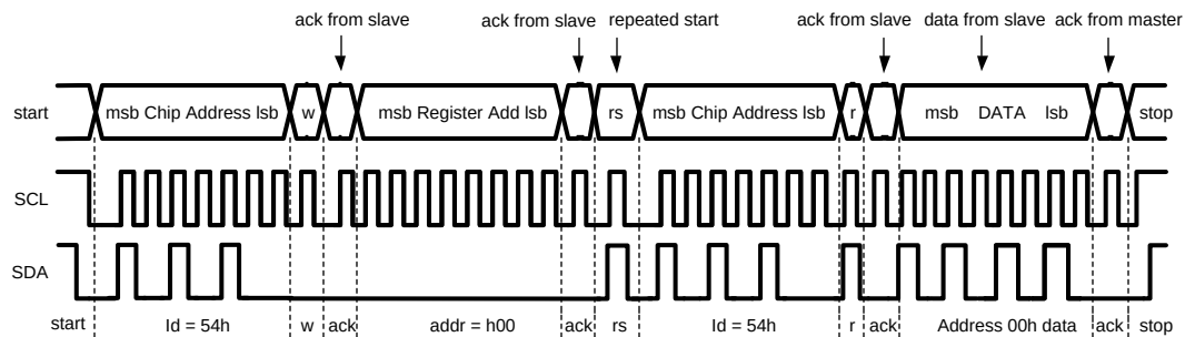
Figure 18. I²C Read Cycle
