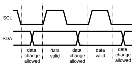
Figure 15. I 2 C Signals: Data Validity
