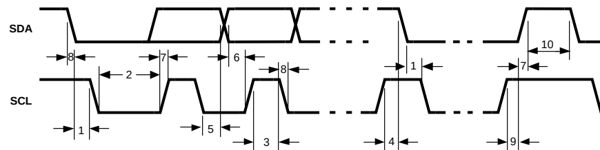
Figure 19. I²C Timing Diagram
