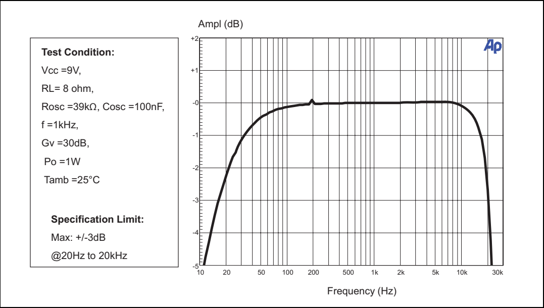
Figure 20. Frequency response
