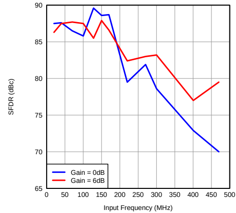
Figure 91. SFDR vs Input Frequency
