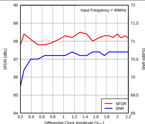
Figure 101. Performance vs Input Clock Amplitude
