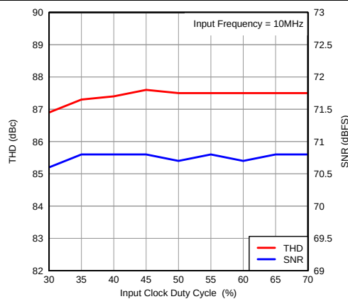
Figure 103. Performance vs Input Clock Duty Cycle
