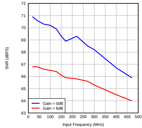
Figure 111. SNR vs Input Frequency (CMOS)
