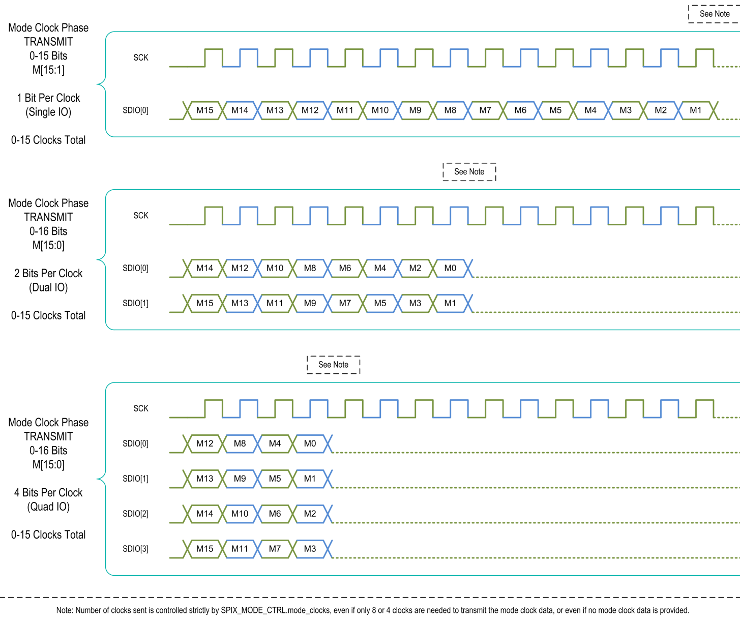
Figure 7.22: SPIX Memory Read - Mode Clock Phase
