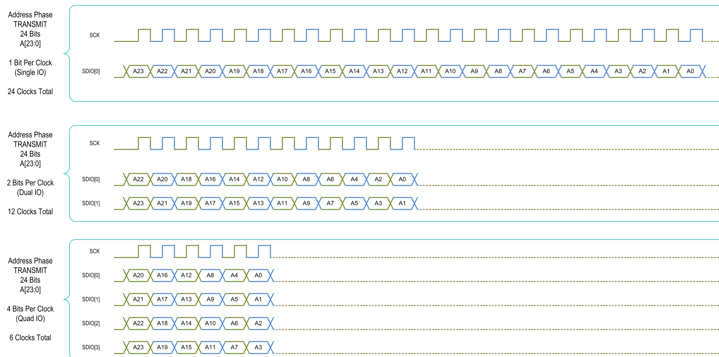
Figure 7.21: SPIX Memory Read - Address Phase
