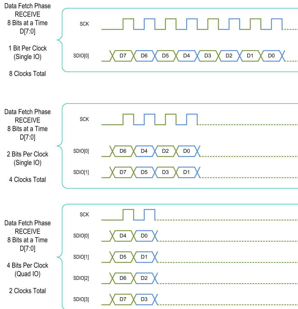
Figure 7.23: SPI XIP Memory Read - Data Fetch Phase
