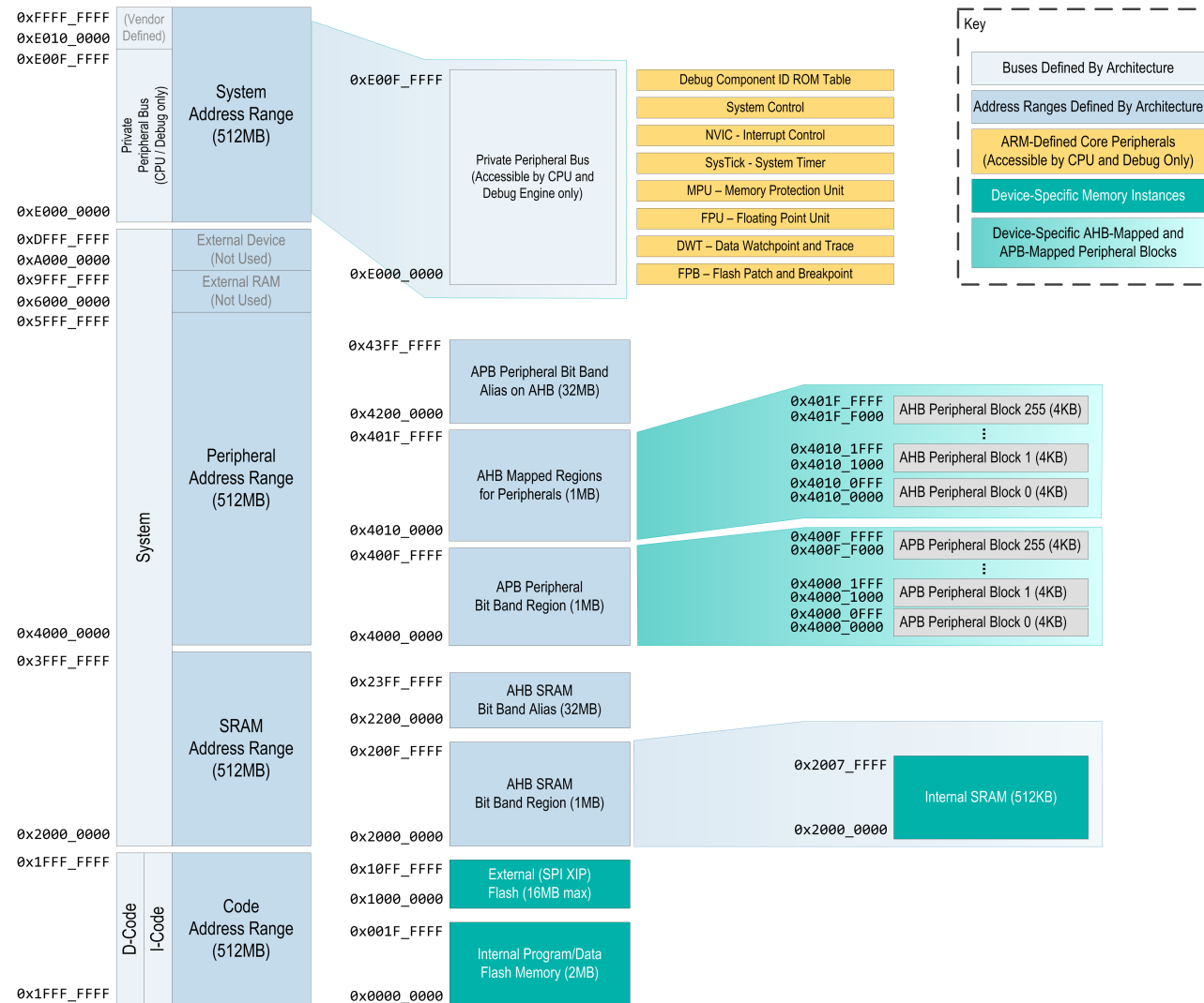
Figure 2.2: Memory Map
