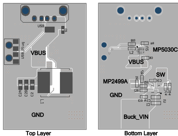
Figure 7: Recommended Layout
