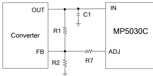
Figure 6: V ADJ Set Maximum V OUT
