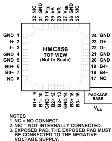
Figure 3. Pin Configuration
