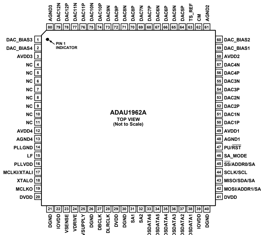
Figure 3. Pin Configuration
