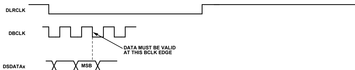
Figure 23. Inverted DBCLK Mode in DAC Serial Data Transmission (Applicable in Stereo and TDM, Useful for High Frequency TDM Transmission)
